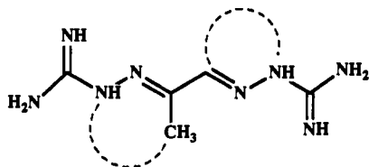
Figure 1. Proposed structural variations of MGBG.
